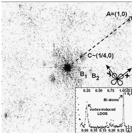
Fig. 2. Power spectrum of the field of view shown in Fig. 1. The atomic periodicity is detected at the four points labeled by A, which by definition are at (0, \pm 1) and (\pm 1, 0) in units of 2\pi/a_0 . The harmonics of the supermodulation are labeled B_1 and B_2 . The signature of the vortex-induced LDOS appears at four k -space points labeled by C. The inset shows a linecut along the dashed line, with Lorentzian fits to the k -space locations of the vortex-induced LDOS and the atomic signature.
