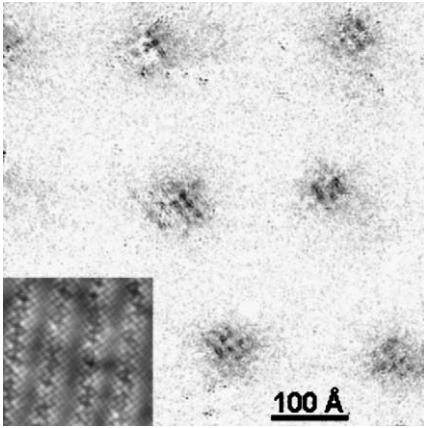
Fig. 1. Map of S_1^2(x, y, 5) : seven vortices are evident as the darker regions of dimension \sim 100 Å with an internal ‘checkerboard’ pattern. The inset shows a topographic image of the BiO plane at 2\times magnification. The atomically resolved square lattice and the supermodulation at 45^\circ are evident.
